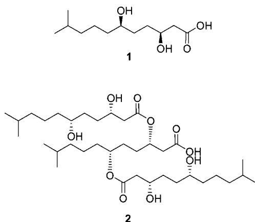
Figure 1. (–)-(3 S ,6 R )-3,6-dihydroxy-10-methylundecanoic acid ( 1 ) and its trimer ( 2 ).
