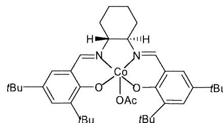
Scheme 1. Reagents and conditions: (i) ( R,R )-(salen)Co III ·OAc (0.5 mol-%), distd. H 2 O (0.55 equiv.), 0 °C, 14 h, (46% for 3a , 45% for 3b ).
