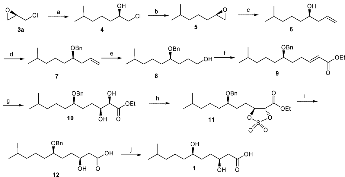
Scheme 2. Reagents and conditions: (a) \text{Me}_2\text{CH}(\text{CH}_2)_2\text{MgBr} , CuI, dry \text{Et}_2\text{O} , -78^\circ\text{C} , 12 h, 98%; (b) KOH, \text{Et}_2\text{O} , 0^\circ\text{C} to room temp., 6 h, 96%; (c) \text{C}_2\text{H}_5\text{MgBr} , CuI, THF, -78^\circ\text{C} to room temp., 12 h, 95%; (d) BnBr, TBAI, NaH, DMF, 0^\circ\text{C} to room temp., 1.5 h, 97%; (e) (i) \text{BH}_3\cdot\text{SMe}_2 , THF, 0^\circ\text{C} to room temp., 4 h; (ii) 3 N NaOH, \text{H}_2\text{O}_2 , 0^\circ\text{C} to room temp., 6 h, 88%; (f) (\text{COCl})_2 , DMSO, \text{CH}_2\text{Cl}_2 , -78^\circ\text{C} , 1.5 h, \text{Et}_3\text{N} , -60^\circ\text{C} , 1 h (ii) \text{Ph}_3\text{P}=\text{CHCO}_2\text{Et} , THF, room temp., 24 h, 93%; (g) (\text{DHQ})_2\text{PHAL} (1 mol-%), 0.1 M \text{OsO}_4 (0.5 mol-%), \text{K}_2\text{CO}_3 , \text{K}_3\text{Fe}(\text{CN})_6 , \text{MeSO}_2\text{NH}_2 , t\text{BuOH}/\text{H}_2\text{O} , 1:1, 0^\circ\text{C} , 24 h, 96%; (h) (i) \text{SOCl}_2 , \text{Et}_3\text{N} , \text{CH}_2\text{Cl}_2 , 0^\circ\text{C} , 30 min; (ii) \text{RuCl}_3 , \text{NaIO}_4 , \text{CCl}_4/\text{MeCN}/\text{H}_2\text{O} , 2:2:3, 0^\circ\text{C} , 1 h, 98%; (i) \text{NaBH}_4 , DMAC, 25^\circ\text{C} , 30 min, then 20% aq. \text{H}_2\text{SO}_4 , overnight, 86%; (j) 20% \text{Pd}(\text{OH})_2/\text{C} , \text{H}_2 , EtOAc, room temp., 10 h, 81%.
